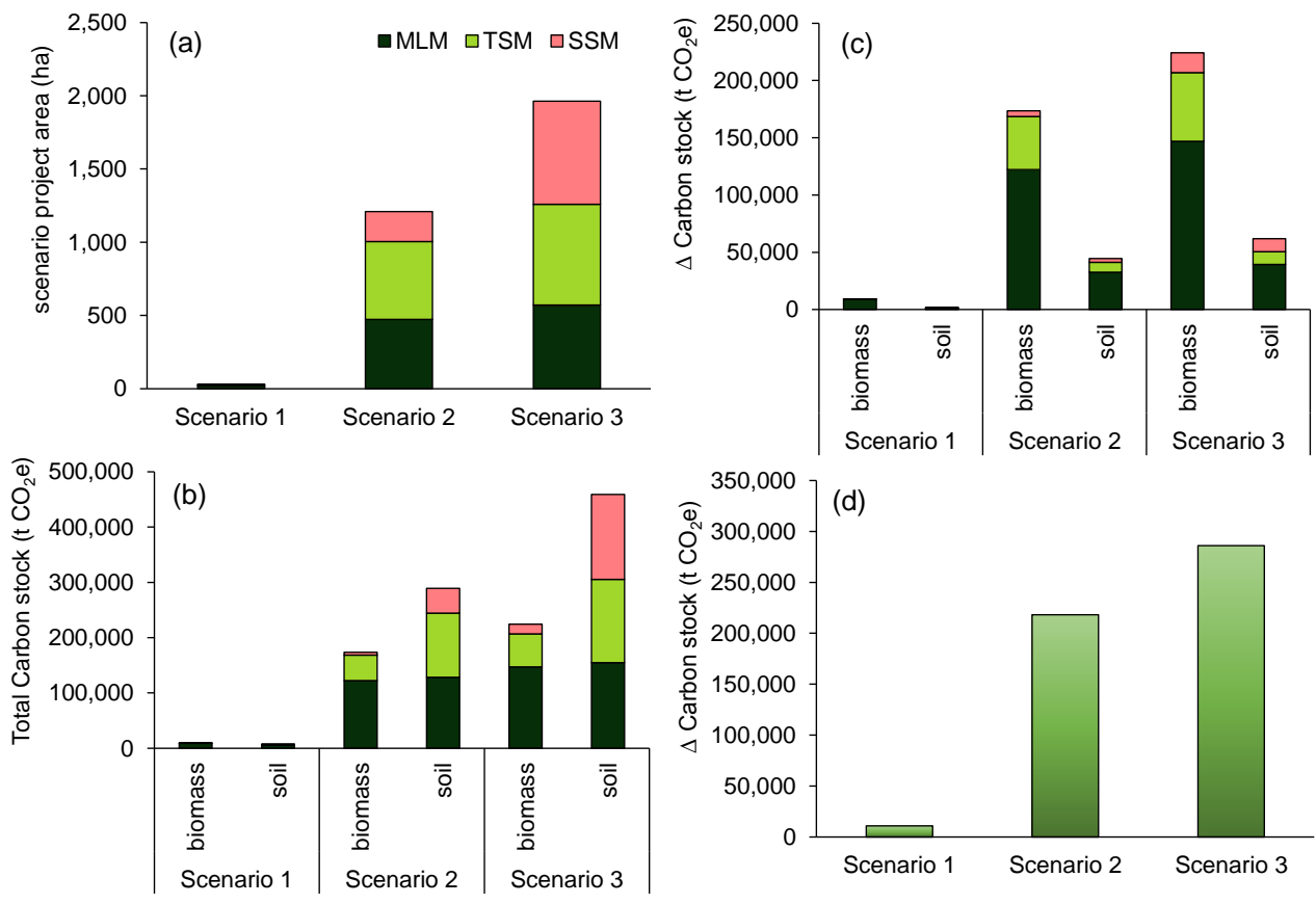
Figure 32. (a) Project area for each scenario considered, and breakdown of the area for each stratum; MLM = Mangrove low marsh, TSM = Tidal saltmarsh, SSM = Supra-tidal saltmarsh. (b) Estimated total carbon stock as t CO 2 e for the respective area of each scenario, based on a 30 year timeframe without sea level rise. (c) Estimated net project benefit from the change in carbon stock as t CO 2 e for the respective area of each scenario, based on a 30 year timeframe without sea level rise. The contribution of soil and biomass carbon pool is indicated separately, as Scenario 3 includes mainly additional supra-tidal elevations with lower and sparse vegetation. (d) Total net project benefit for the combined soil and biomass carbon stock change subject to each scenario activity.
