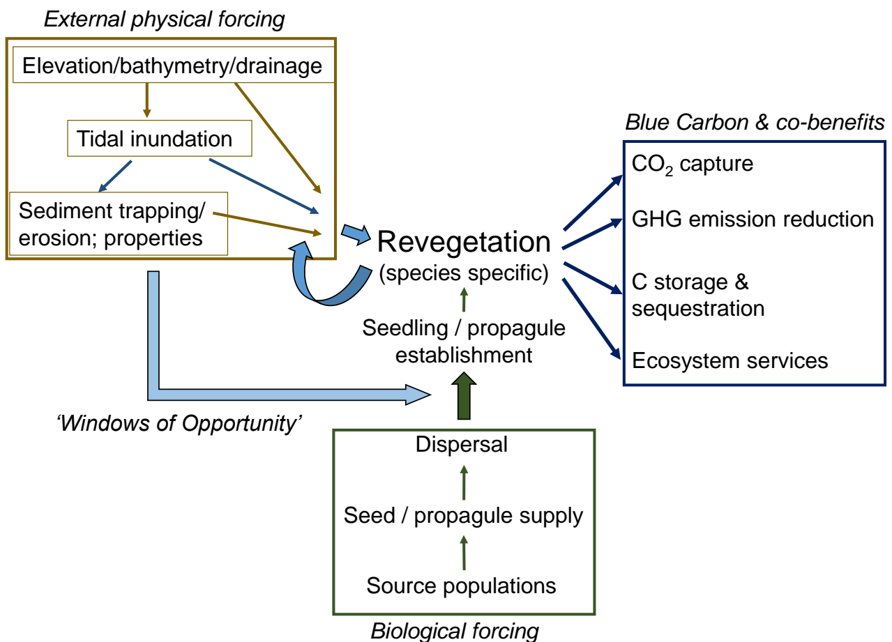
Figure 2. Conceptual diagram of processes enabling Blue Carbon benefits through tidal re-connection of a salt pond.
