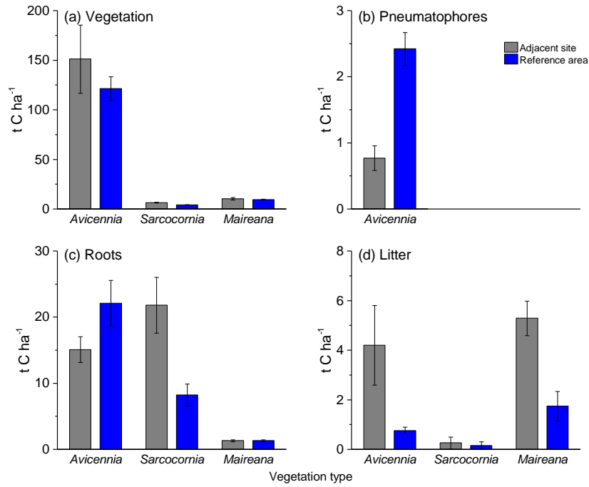
Figure A.5. Carbon pools (mean \pm 1SE) of (a) vegetation, (b) pneumatophores, (c) roots and (d) litter for the vegetation types: Avicennia marina mangrove forest, Sarcocornia quinqueflora saltmarsh, and Maireana oppositifolia shrubland, separated by the area adjacent (outside) of the trial pond, and a reference area near St Kilda.
