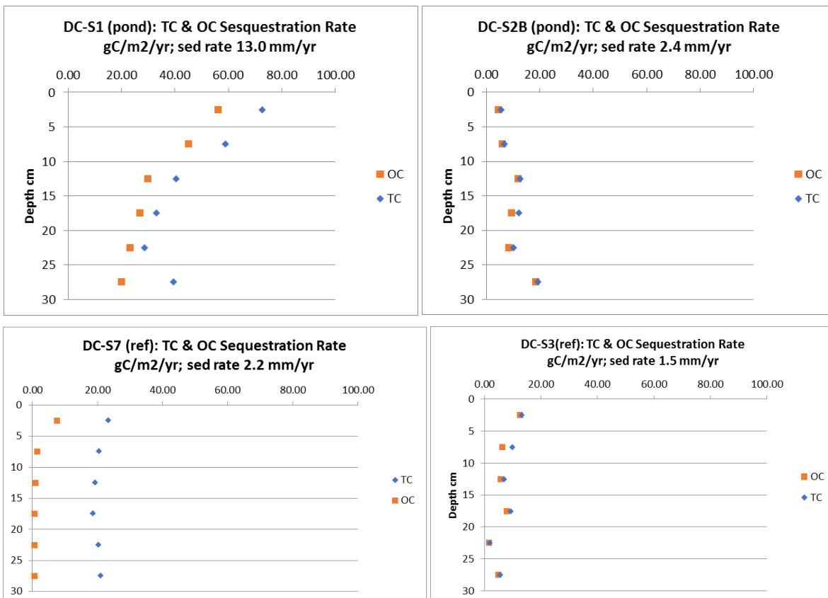
Figure A.2. Carbon sequestration rates for total carbon and organic carbon for the drained pond sites DC-S1 and DC-S2B and reference sites DC-S3 and DC-S7.
