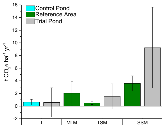
Figure 15. Fluxes of CO 2 e (average ± SE) across the strata in the trial pond, control pond and reference area. The elevation strata were I= inundated, MLM=Mangrove low saltmarsh, TSM=Tidal saltmarsh, and SSM=Supra-tidal saltmarsh.
